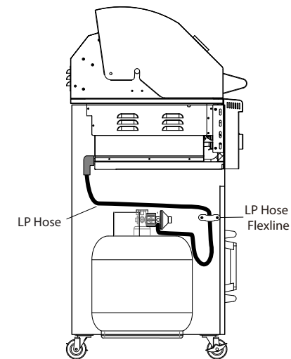
Liquid Propane (LP) Installation
